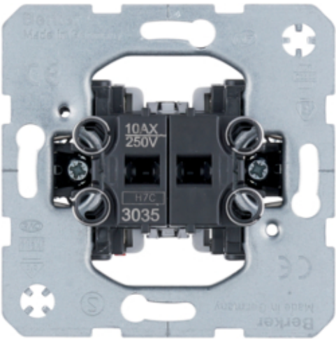
Doble interruptor on/off 10AX, 250V
